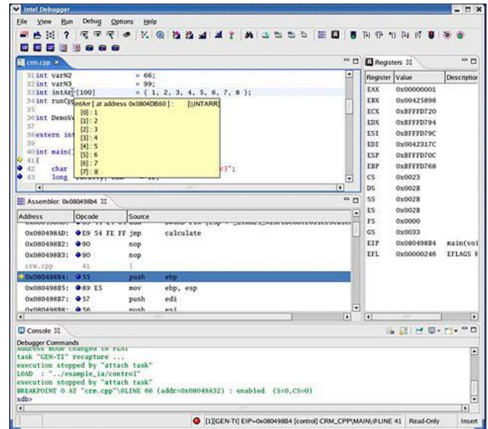
The JTAG and Application Debuggers provide an Eclipse-based GUI running on Linux* host.
